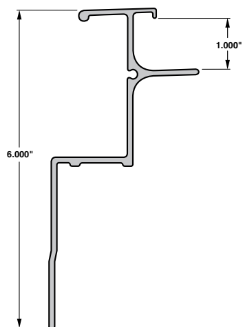
Top Rail 1.000" GVSD
