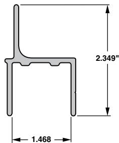
Front Top Connector GVSD – Pre 2003
