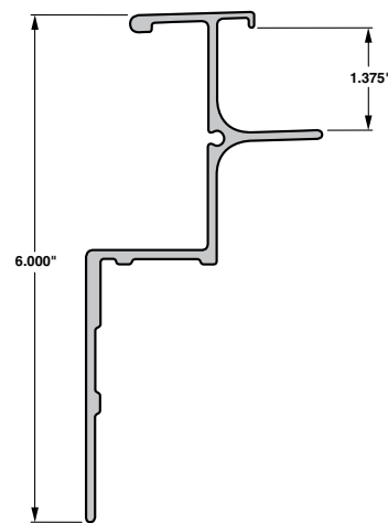
Top Rail 1.375" GVFD
