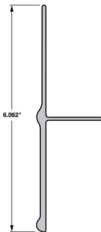
Bottom Rail GVFD 1997 and Newer
