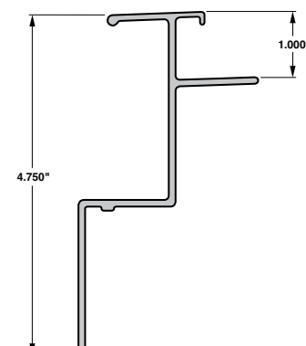
Top Rail Roof Bow GVFD
