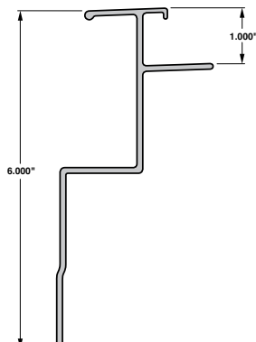
Top Rail Roof Bow GVSD
