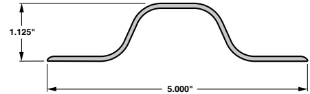
Rub Rail – Rounded Style
