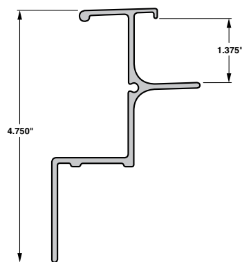
Top Rail 1.375" GVFD
