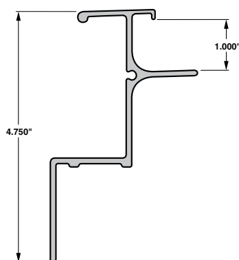
Top Rail 1.000" GVFD
