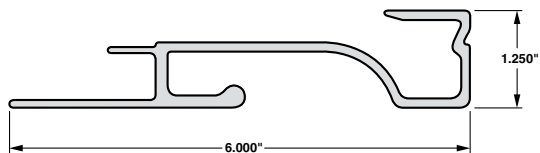
Reefer Door Post L/S Current
