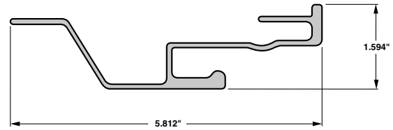
Side Door Post L/S
